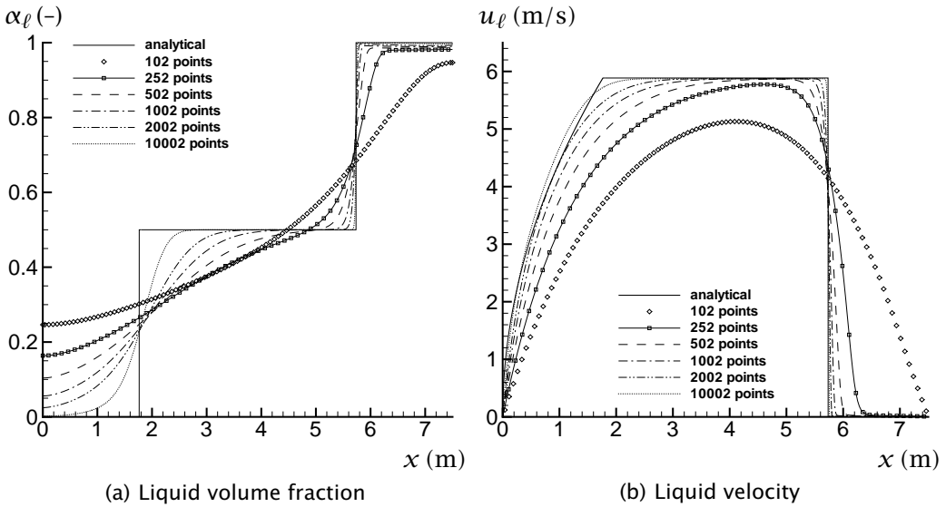
Figure 4.6: Water-air separation at t = 0.6 s. Grid and time-step refinement for the FORCE scheme. C = 0.5 .
