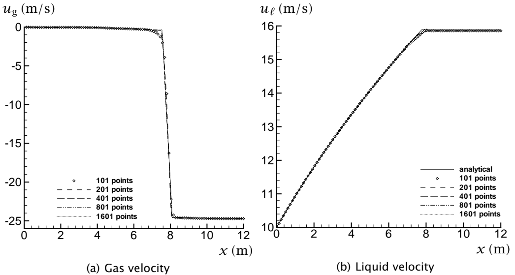
Figure 3.5: Velocities for the water faucet. Grid convergence of the Roe4 method.
